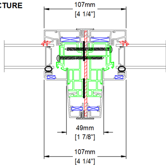
FLAT PLATE STEEL MULL
