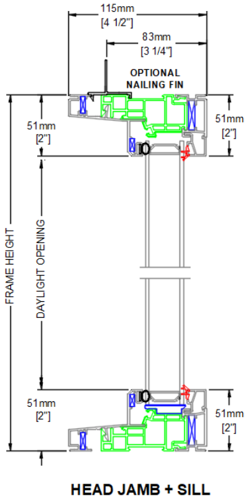
31.75mm (1 1/4 ") DUAL PANE GLASS
