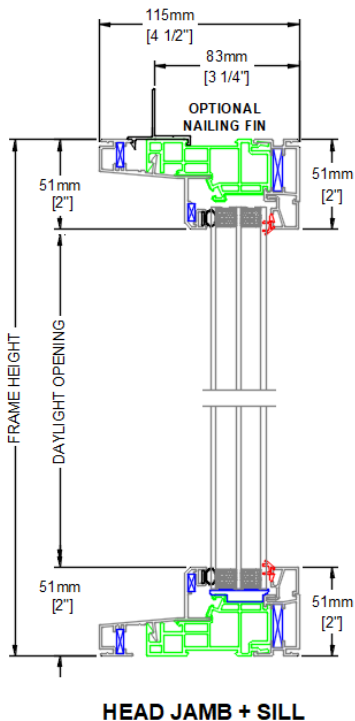
31.75mm (1 1/4 ") TRIPLE PANE GLASS
